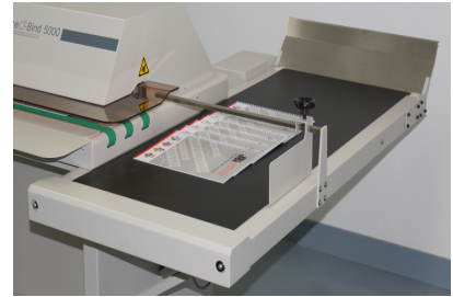
Optional 500mm wide conveyor with a capacity of up to 100 books bound in 1/4 inch
